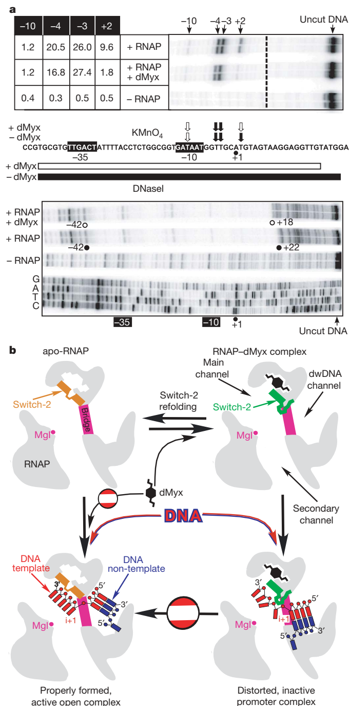
Figure 3 | A mechanism of the dMyx action. a , Myx alters the contacts between RNAP and \lambda P R promoter DNA. a , A linear DNA fragment encompassing positions -81 to +70 of the \lambda P R promoter was generated by polymerase chain reaction (PCR); the non-template DNA strand was end-labelled with [ 32 P]- \gamma -ATP (see Methods). The sequence from -44 to +23 is shown. The -35 and -10 hexamers are indicated by black boxes, the start site (+1) is shown by a black dot. The top panel shows probing of the non-template strand by piperidine-induced cleavage of the permanganate-modified T residues. Reactivities of -10, -4, -3 and +3 residues (quantification described in Methods) are shown to the left of the gel and summarized above the promoter sequence where black and white arrows indicate high and low reactivity, respectively. The bottom panel shows protection of the non-template DNA strand from DNaseI digestion. The footprint boundaries in the promoter region shown are indicated on the gel and by black (RNAP alone) and white (RNAP with the inhibitor) bars below the promoter sequence; the dideoxy-sequencing ladder is shown for reference. In the gels shown, independent reaction repeats were analysed for consistency. b , Schematic drawing of the putative mechanism of the dMyx action. dwDNA, downstream DNA.
