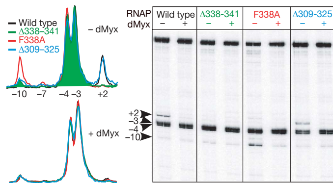
Figure 4 | Mutations in switch-2 affect the open complex formation. Accessibility of the non-template DNA (blue) strand residues to permanganate modification probed as in Fig. 3a. Wild-type and mutant RNAPs differ in their patterns of reactivity in the absence of dMyx (top traces) but are nearly identical in the presence of 10 \mu M dMyx (bottom traces). Notably, \beta' \Delta 309-325 that removes the entire rudder loop (which is inserted in the same helix as switch-2, but is unlikely to interfere with the nucleic acids) has no effect on DNA melting, suggesting that a melting defect of a different rudder deletion 19 might be due to changes in the adjacent switch-2 instead.
